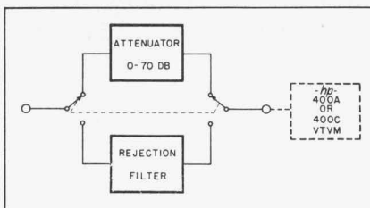
Figure 7. Block diagram of circuit of -hp- Model 320 Distortion Analyzer.
